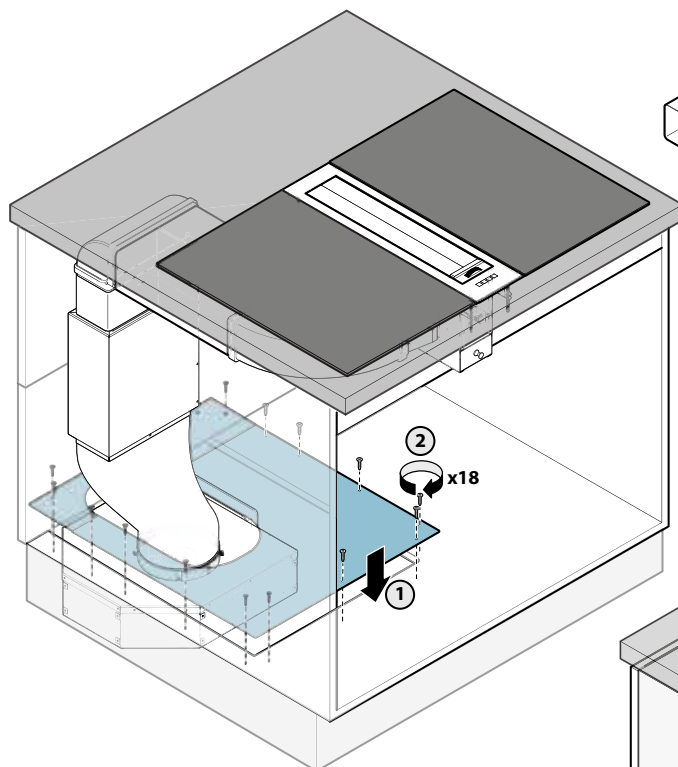
INSTALLAZIONE A PARETE CAPP A PIANO DOUBLE SUCTION PIANO DOUBLE SUCTION HOOD WALL INSTALLATION
